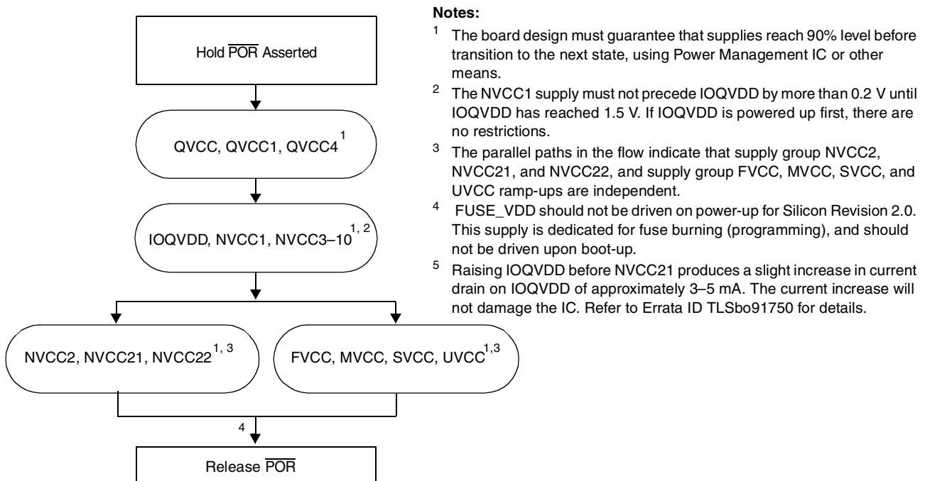
Figure 2. Option 1 Power-Up Sequence for Silicon Revision 2.0
